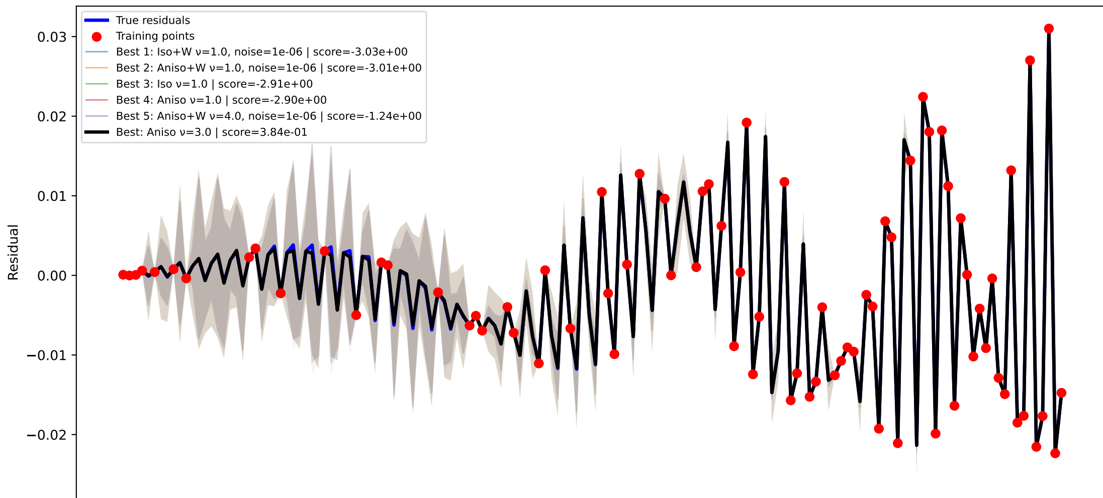
GPR kernel comparison node=51 RMSE=1.691e-04, train RMSE=1.461e-11
